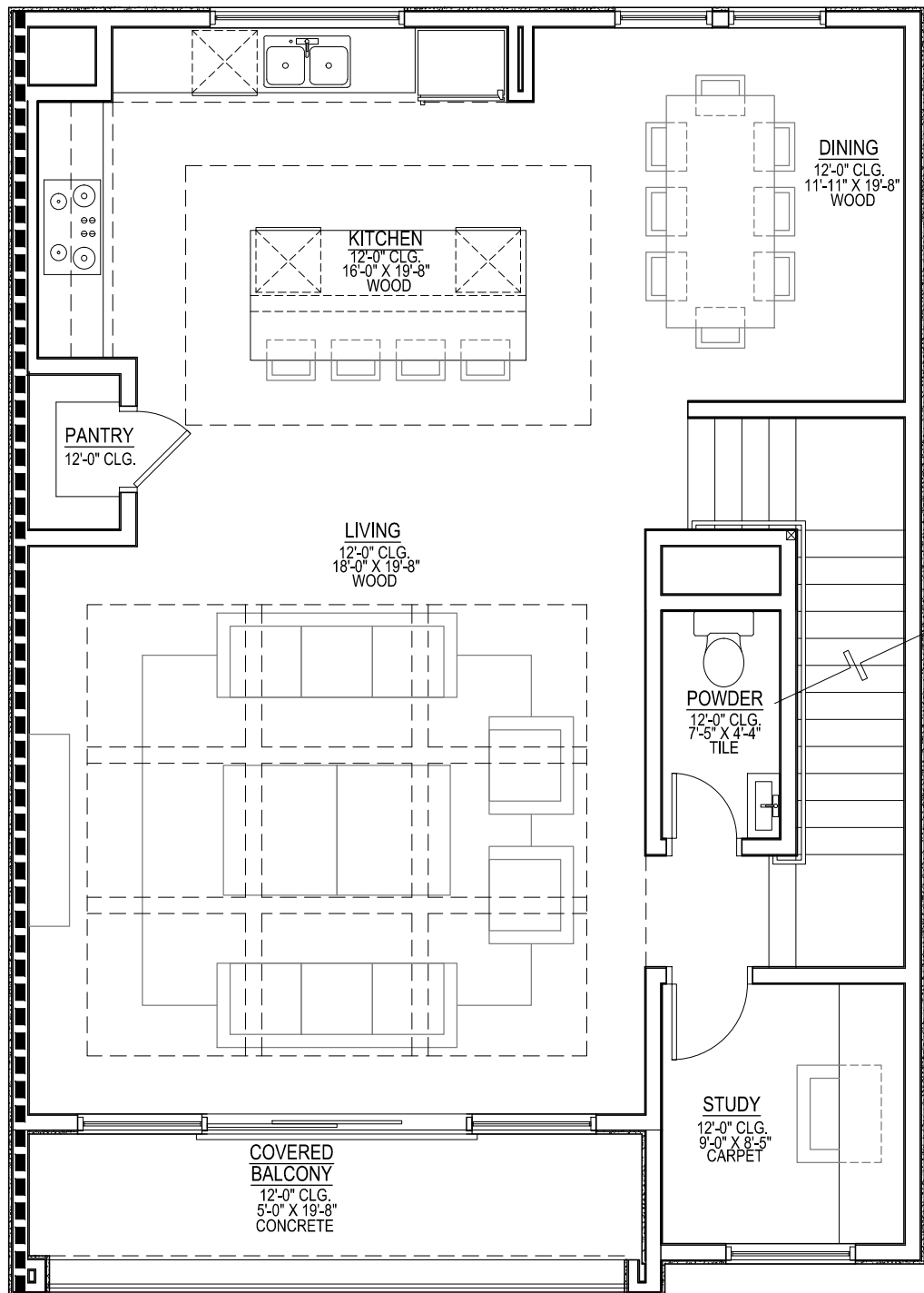
2 SECOND FLOOR PLAN
